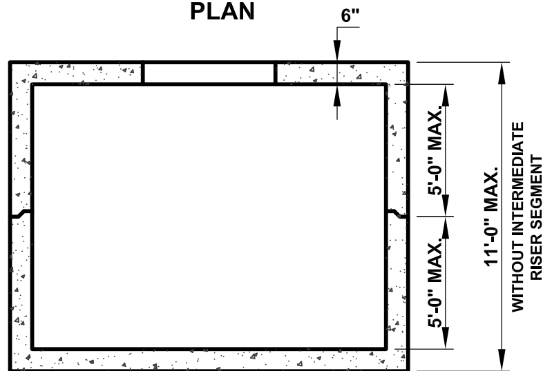
SECTION
